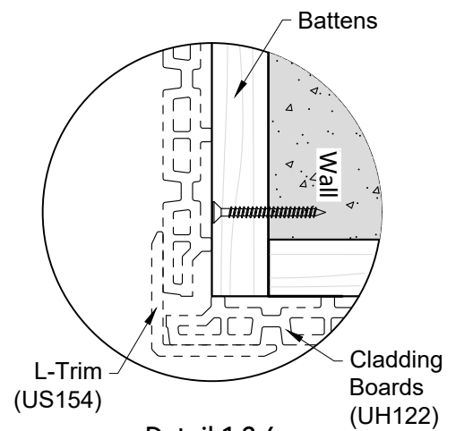
Detail 1.2.4
