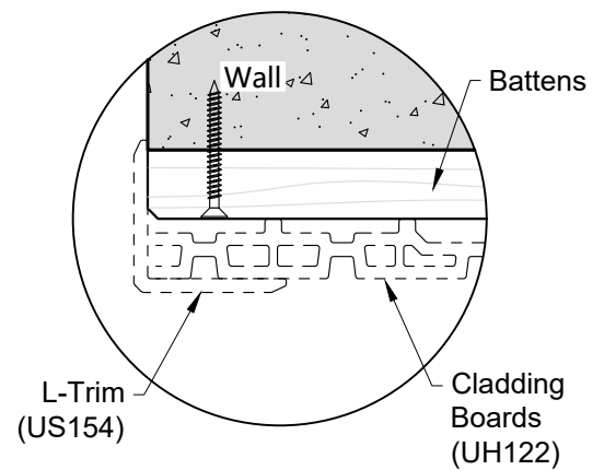
Detail 1.2.3
