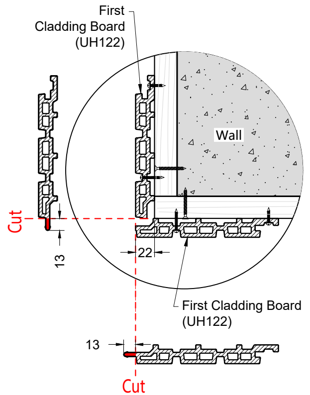
Detail 2.1.1
